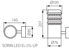
SORIN LED EL-21L-UP
