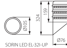
SORIN LED EL-32I-UP
